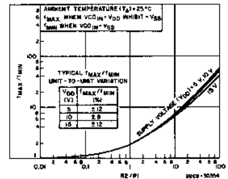
Fig. 8 — Typical t_{MAX}/t_{MIN} as a function of R_2/R_1 .
